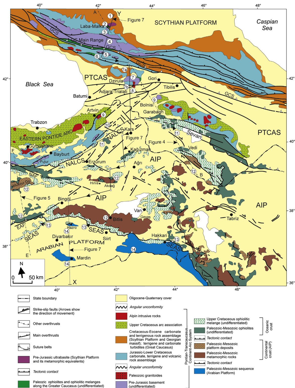
Figure 1. Sketch Geological map depicting the terranes of the Caucasus north-central Middle-East region. NAF: North Anatolian Fault, EAF: East Anatolian Fault, AIP: Anatolian-Iranian platform, PTCAS: Pontian-Transcaucasus Continent-Arc System, GCS: Greater Caucasus Suture, NALCS: North Anatolian-Lesser Caucasus Suture, SEAS: Southeastern Anatolian Suture (from numerous sources). Encircled numbers indicate place of logs cited in the text.
