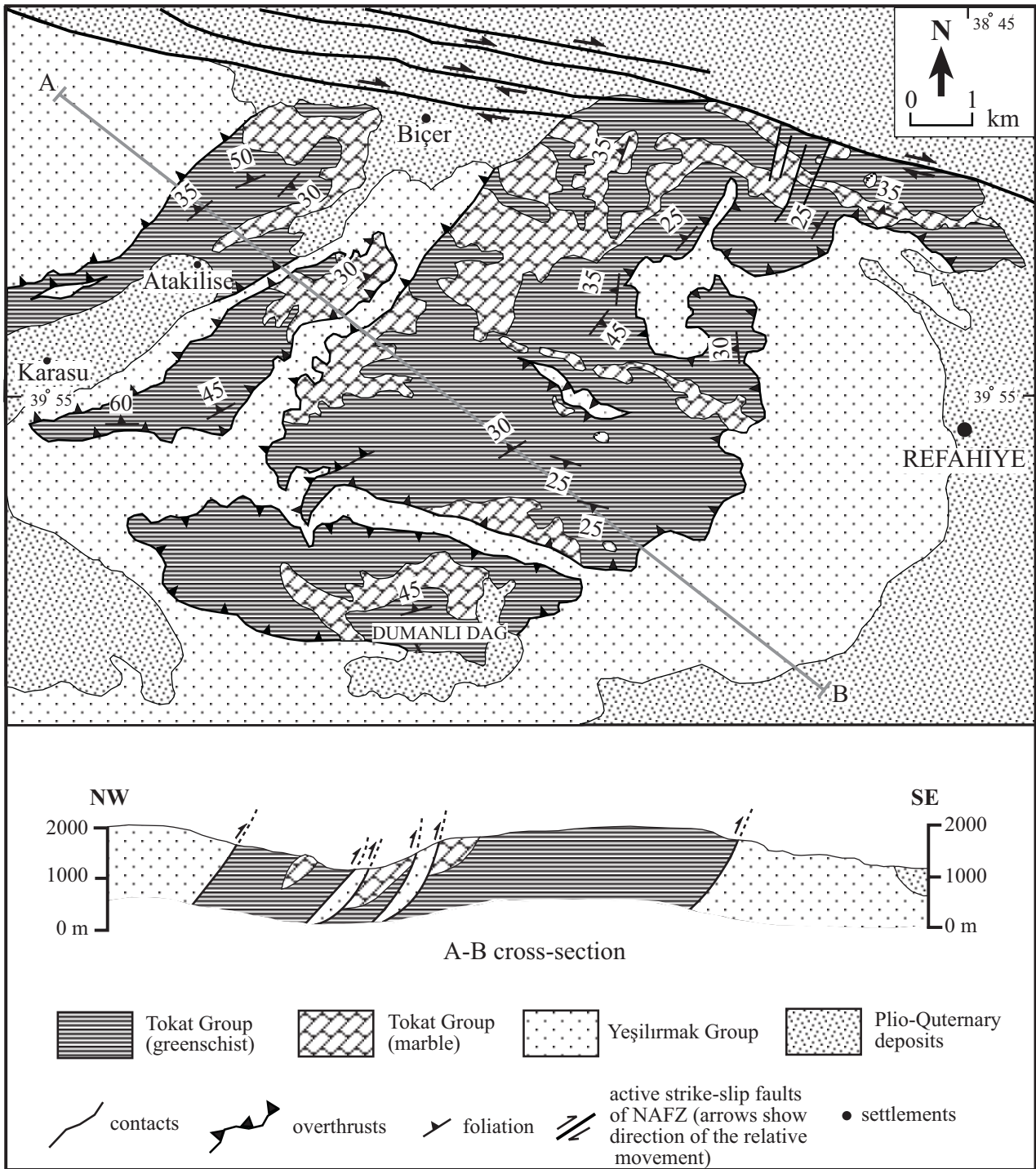
Figure 5. Geological map of Dumanlı Dağı of Refahiye area (after A. Yılmaz et al. 1985b). For location see Figure 2.
