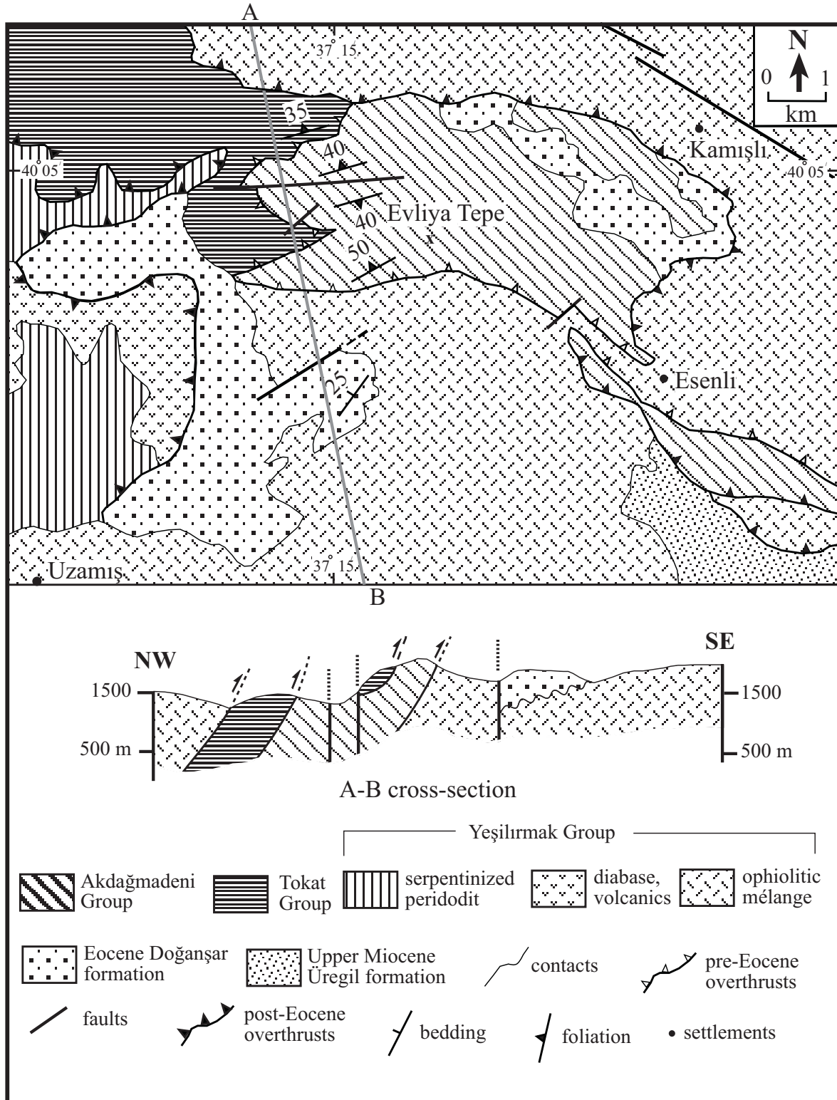
Figure 6. Geological map of the Evliya Tepe area showing relationship between Tokat Group, Akdağmadeni Group and Yeşilırmak Group (after A. Yılmaz 1982b). For location see Figure 2.
