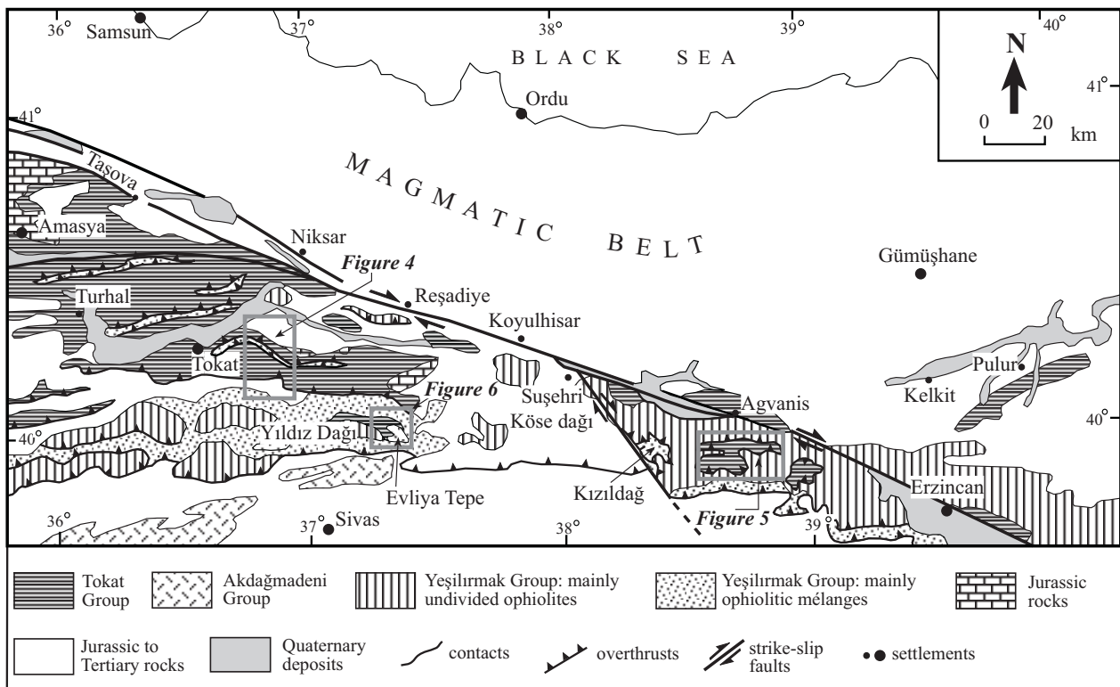
Figure 2. Simplified geological map of the area between Tokat, Sivas and Erzincan (after A. Yılmaz 1980, 1982b; Özcan et al. 1980; Özcan & Aksay 1996; and our own observations). Insets show the location of the maps displayed in the following figures.
