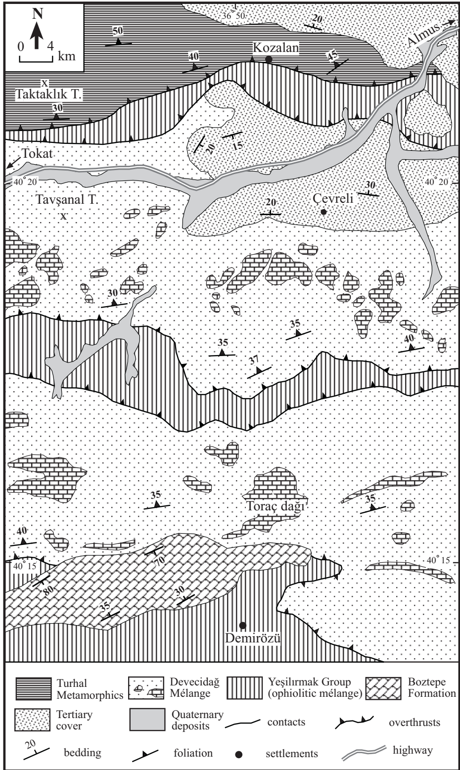
Figure 4. Geological map of the area between Tokat and Almus (after A. Yılmaz 1980, 1982b; Özcan & Aksay 1996; and our own observations). For the location see Figure 2.
