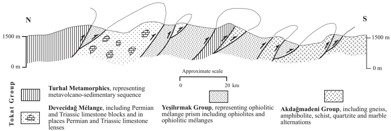
Figure 3. Columnar section indicating structural relationships between Yeşilirmak group, Tokat Group and Akdağmadeni group.
